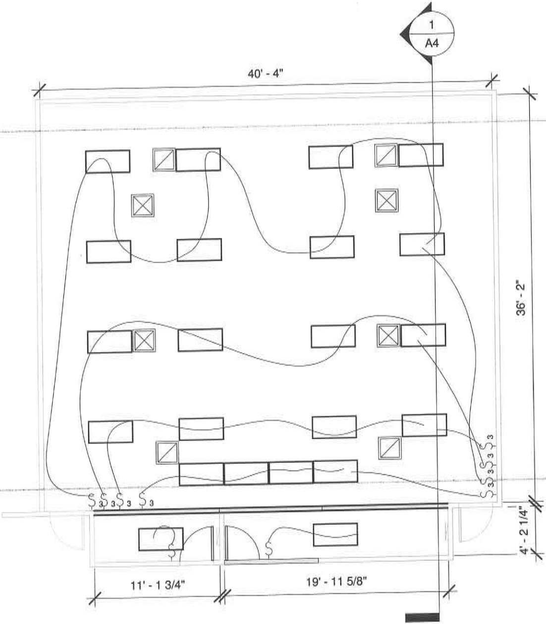
① Lighting Plan 1/8" = 1'-0"
